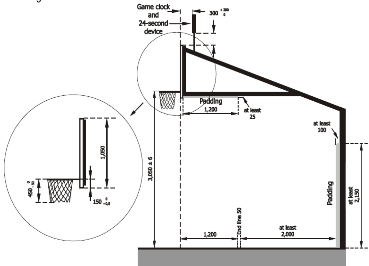
Diagram 1 Backstop unit
